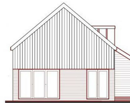
West Elevation
